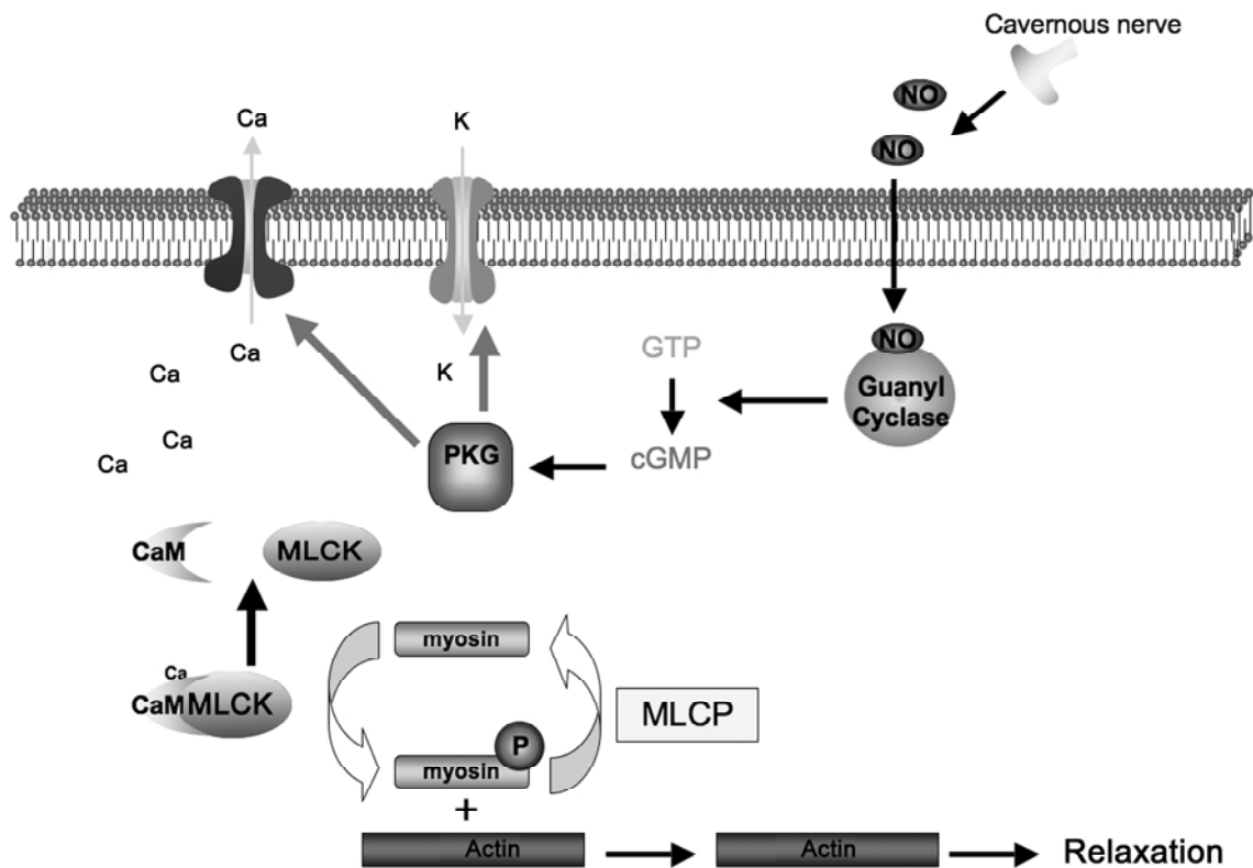
Figure 4. Signaling pathways leading to cavernous smooth muscle (CSM) relaxation. Sexual stimulation triggers the release of nitric oxide (NO) from cavernous nerves in the penis. NO diffuses into CSM cells (CSMC) and activates guanyl cyclase, which then catalyzes the conversion of guanosine triphosphate (GTP) to cyclic guanosine monophosphate (cGMP). cGMP activates protein kinase G (PKG), which in turn phosphorylates potassium (K) and calcium (Ca) channels. Phosphorylation of K and Ca channels leads to an increase of potassium efflux, a reduction of calcium influx, and the dissociation of calcium from calmodulin (CaM), which in turn dissociates from the myosin light chain kinase (MLCK), thus inactivating it. Inactivation of MLCK and removal of phosphates by myosin light chain phosphatase (MLCP) lead to dissociation of myosin from actin and relaxation of actin.
