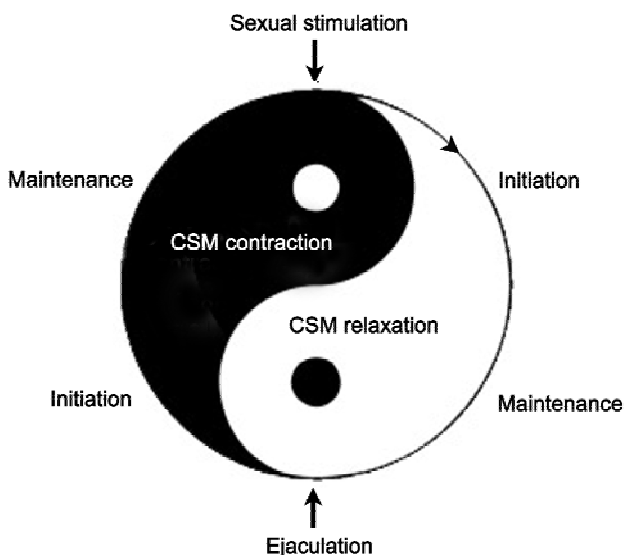
Figure 1. The erection cycle. Erection is initiated by sexual stimulation and maintained during continuous sexual stimulation. Erection starts to subside at ejaculation and the subsequent flaccidity is maintained until the next sexual stimulation. CSM, cavernous smooth muscle.
